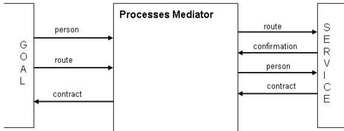
Figure 2. Web Service - G3 interaction
