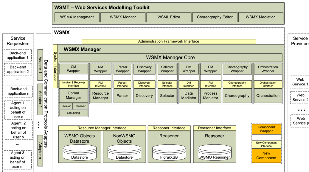
Figure 1: WSMX Architecture
