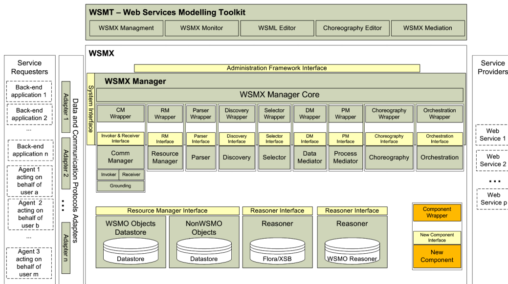
Figure 1: WSMX Architecture
