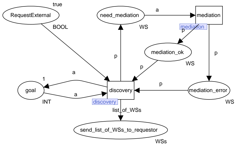
Figure 7: Overview of list of Web Services fulfilling given Goal
