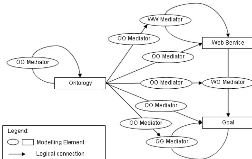
Figure 4. Illustration of mediators in WSMO
